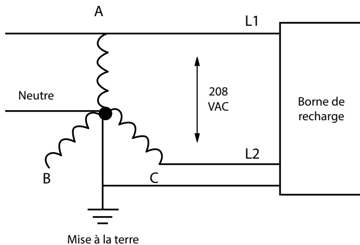
Figure 1 : Triphasé 120/208 VAC
